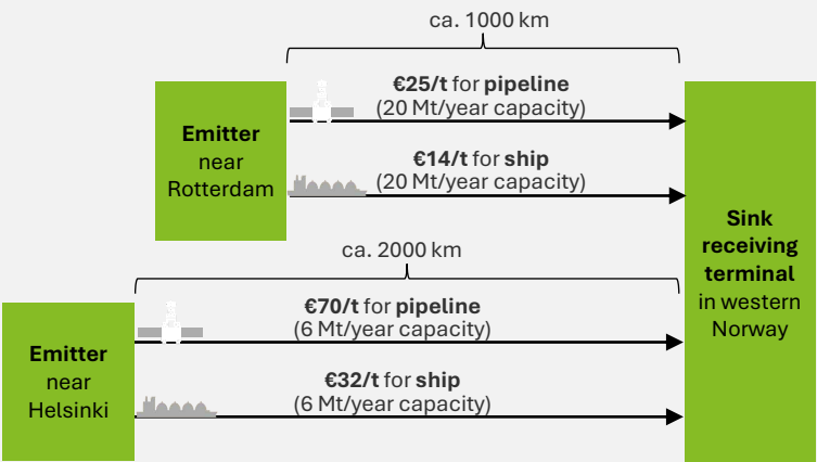
CO 2 transport cost comparison (indicative) 1
