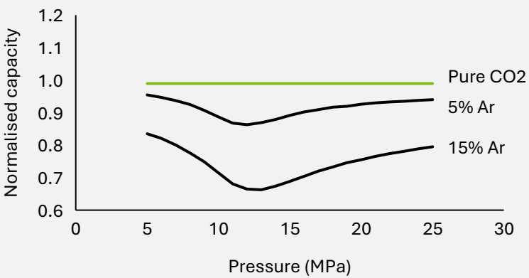
Normalised capacity for different CO 2 purity levels, per pressure level (MPa) 2
