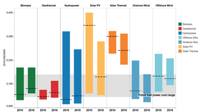
Fig. 4 Levelised Cost of Electricity 2010-2016
