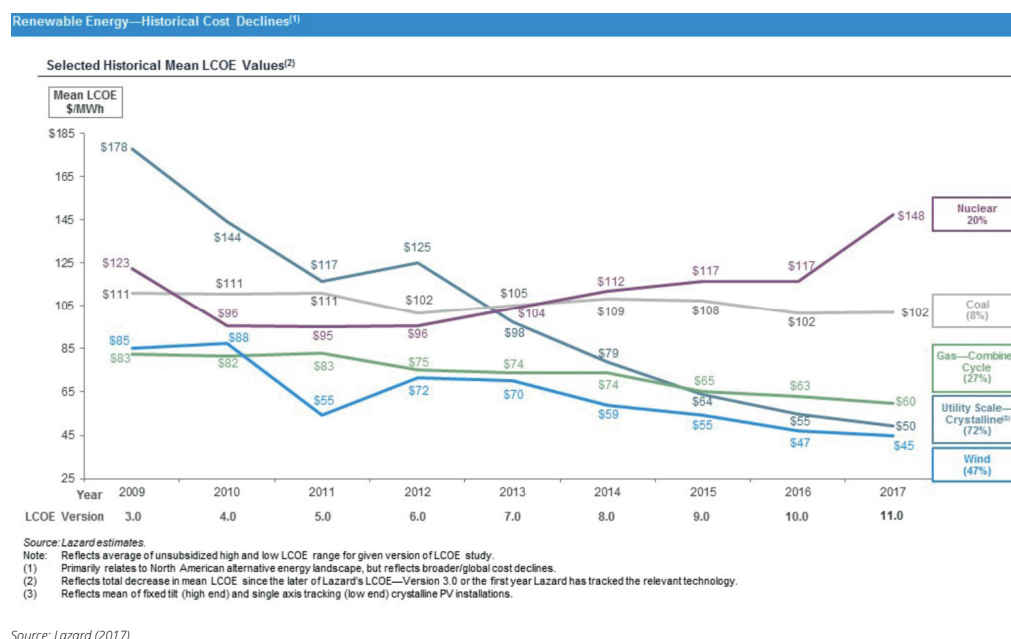
Fig. 5 Historical evolution of LCOE by technology
