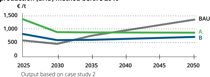
Figure 04. Both clean technologies outperform the conventional production (BAU) method before 2040
