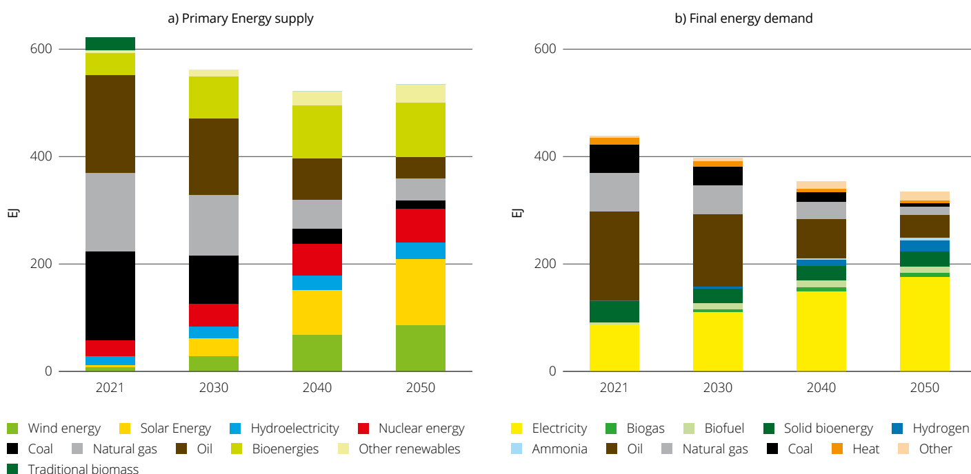
Figure 8. Global primary and final energy mix aligned with net-zero through 2050
