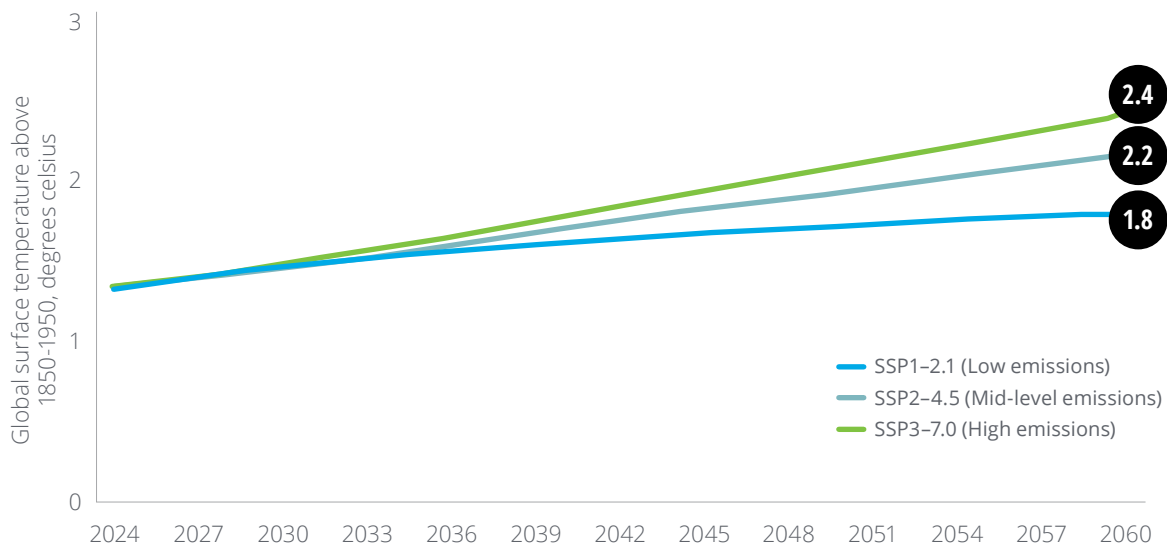
Chart 2.1: Global surface temperature changes under select IPCC SSP scenarios
