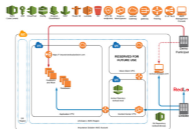
InsureCloud: On-Demand Insurance Platform
